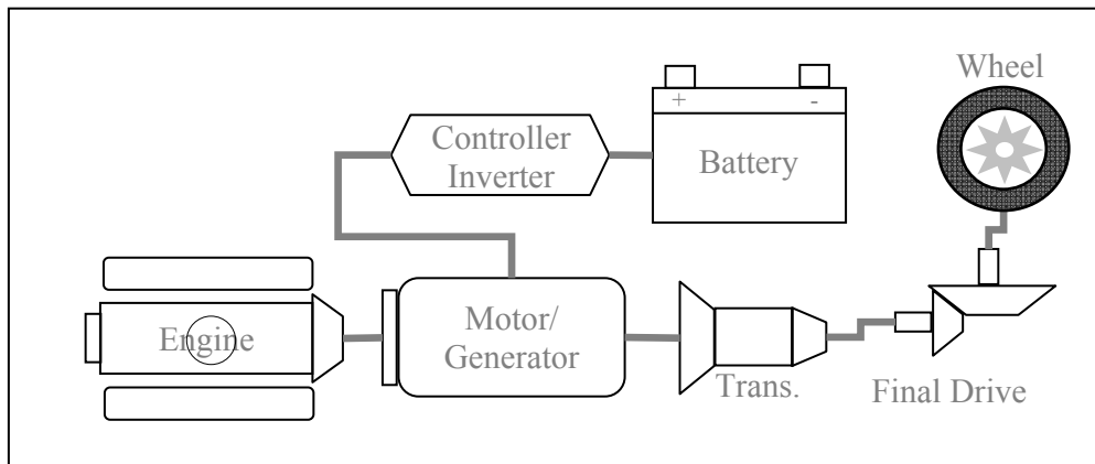
Figure V-14 Schematic of Honda IMA System [Husted, 2003]
